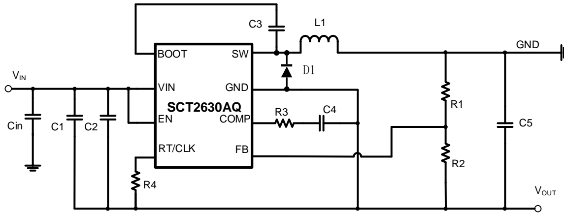
Figure 12. SCT2630AQ Inverting Power Supply
