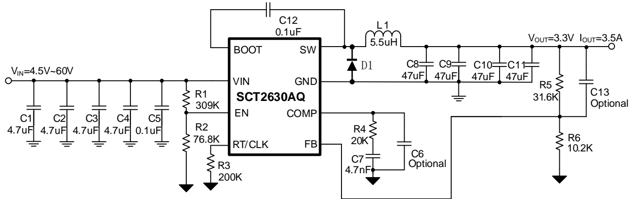
Figure 11. SCT2630AQ Design Example, 3.3V Output with Programmable UVLO
