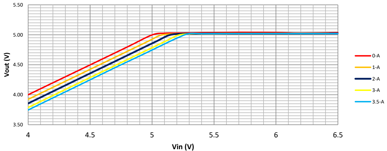
Figure 10. LDO Operation Characteristic ( V_{out} = 5V )
