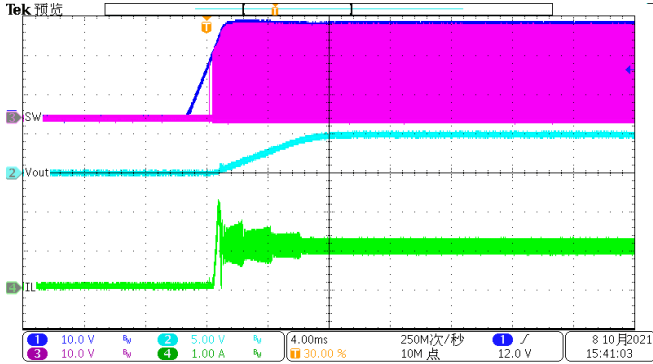
Figure 11. Power up(Iload=1A)
