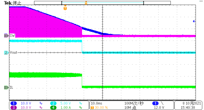
Figure 12. Power down(Iload=1A)
